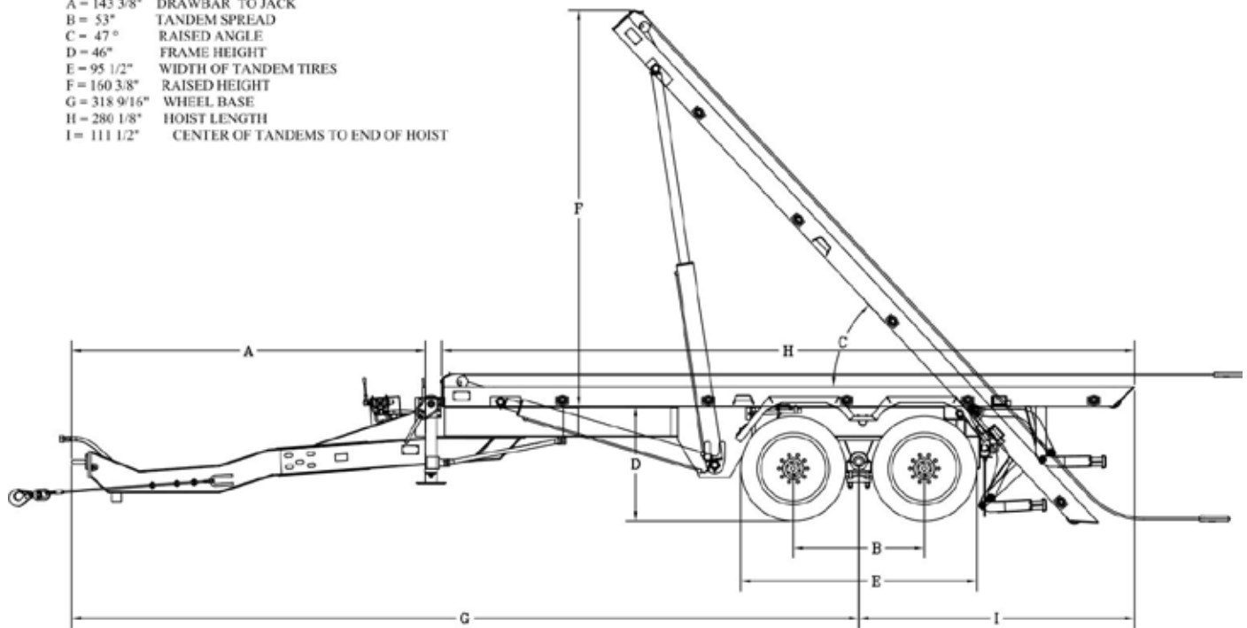
HOIST FRAME DETAIL
