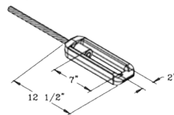
SWIVEL CABLE END
